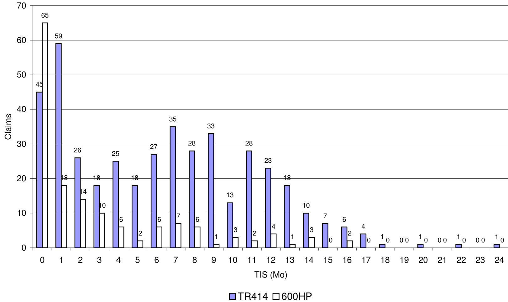
Valve Stem AWS Claims Vs TIS - July 2006 Thru April 2008 Ford North American Vehicle Lines (Except MKX/Edge)
