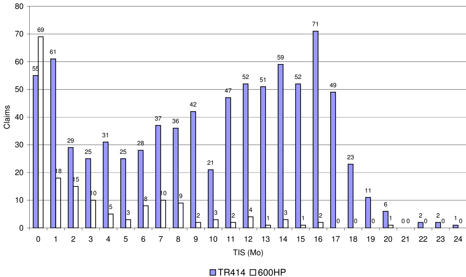
Valve Stem AWS Claims Vs TIS - July 2006 Thru July 2008 Ford North American Vehicle Lines (Except MKX/Edge)
